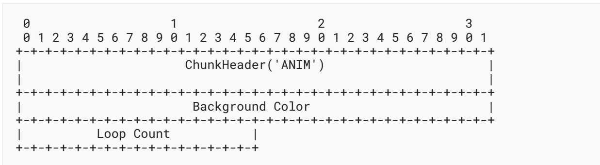
Figure 8: 'ANIM' Chunk
