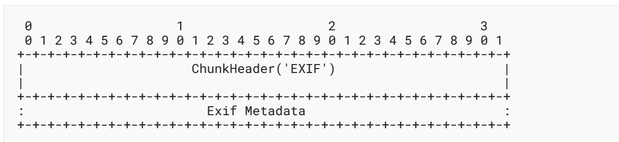
Figure 13: 'EXIF' Chunk
