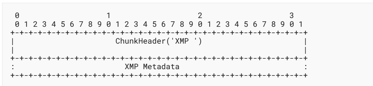
Figure 14: 'XMP ' Chunk
